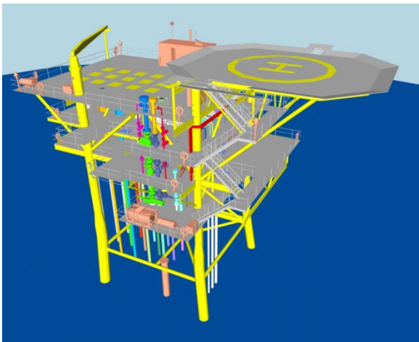
Topsides on the wellhead platforms were designed to comply with API RP 14C. Personnel access is via helicopter
