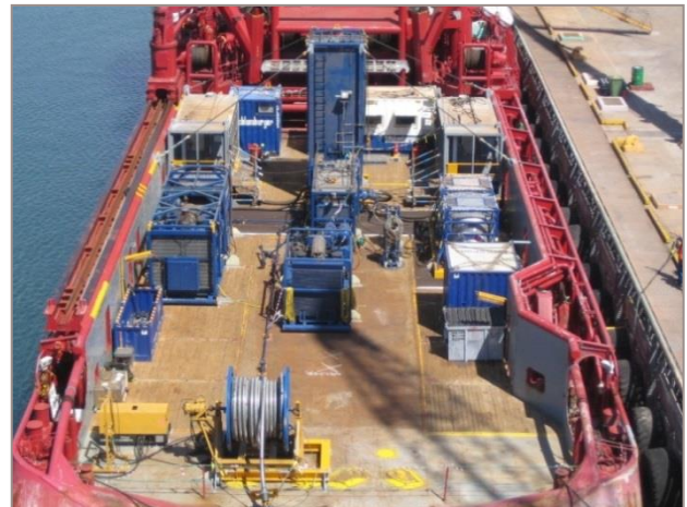
Deck Layout on ‘Far Stream’
